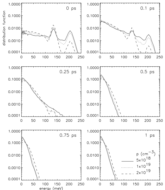
Fig. 10. Temporal evolution of the electron distribution function f_e at six different delay times for three different doping concentrations and T = 77 K.
