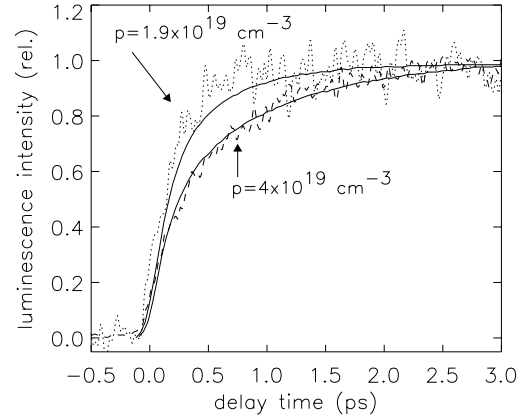
Fig. 3. Time evolution of the luminescence intensity at 13 meV above the renormalized band edge for sample D ( p = 1.9 \times 10^{19} \text{ cm}^{-3} ) and sample F ( p = 4 \times 10^{19} \text{ cm}^{-3} ) at the lattice temperature of 77 K. The solid lines show the results of the Monte-Carlo simulations.
